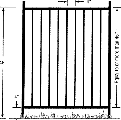
Figure 1 Minimize the size of openings when constructing a barrier.
